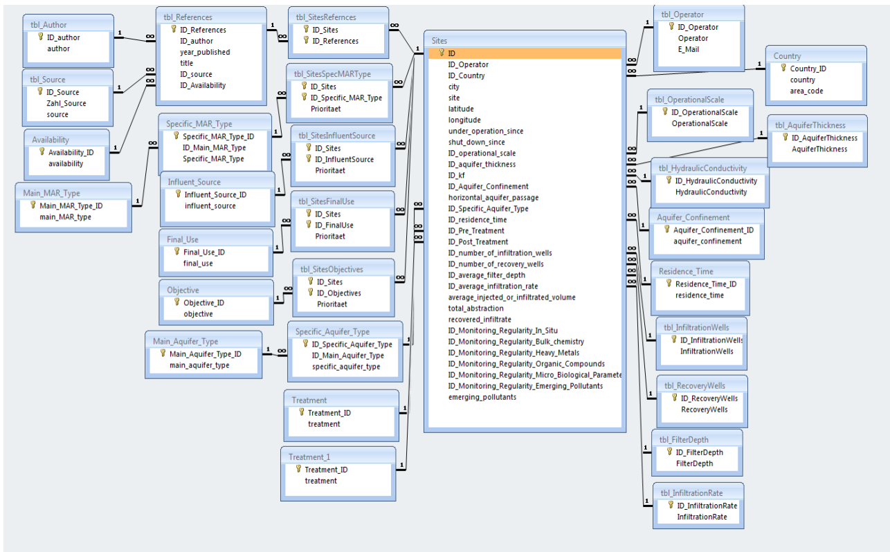
Figure 1: Structure of the MAR database and table relationships
