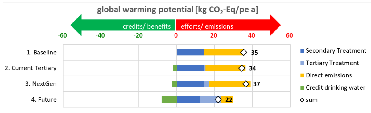
Figure 30: Global warming potential for the Tossa de Mar WWTP & WRP
