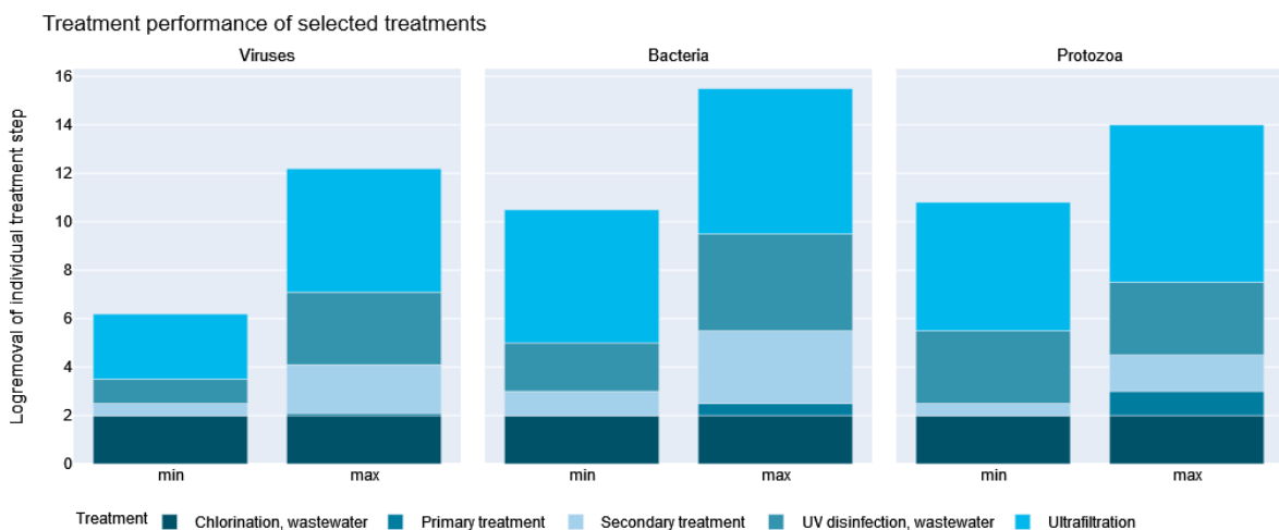
Figure 73: Overview of applied LRVs in the NEXTGEN scenario
