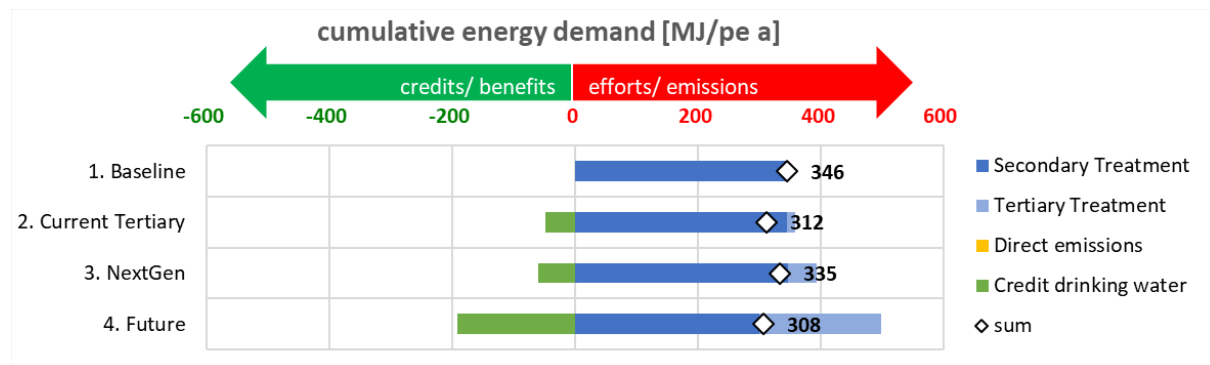
Figure 29: Non-renewable cumulative energy demand for the Tossa de Mar WWTP & WRP
