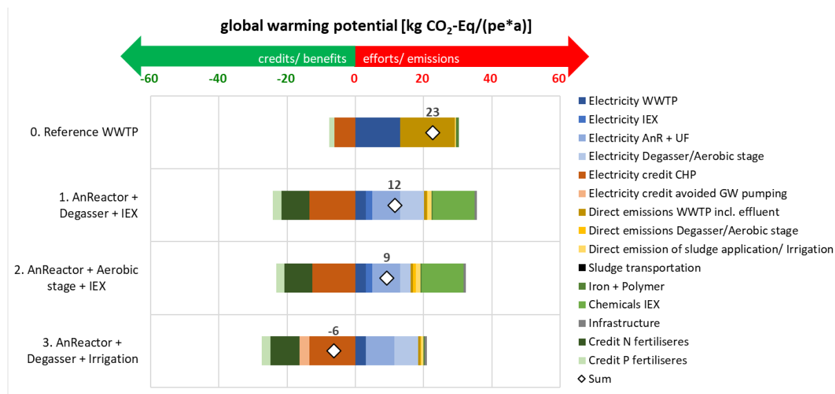
Figure 48: Global warming potential for conventional and NEXTGEN scenarios in Sernal LCA
