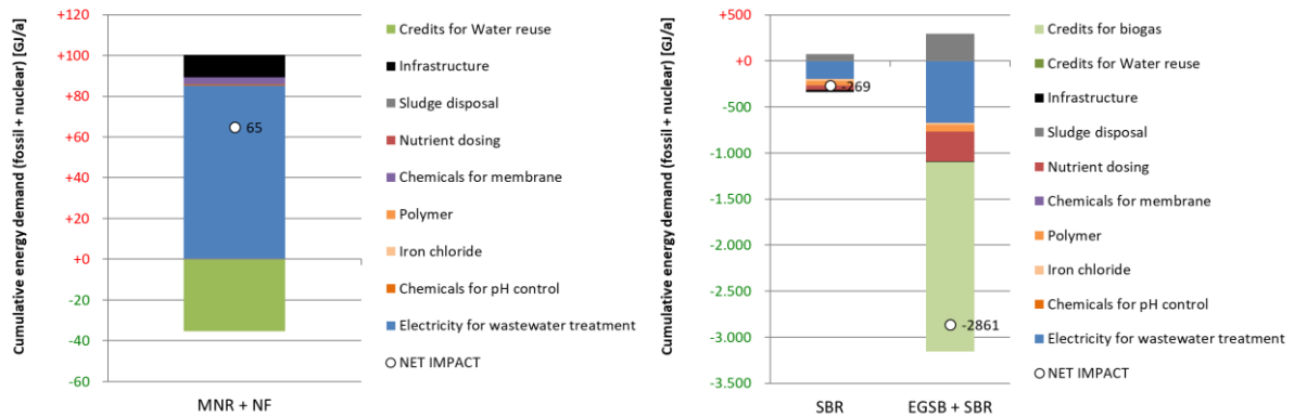
Figure 38: Changes in cumulative energy demand compared to MNR scenario for LaTrappe brewery (left: MNR+NF, right: SBR and EGSB+SBR)
