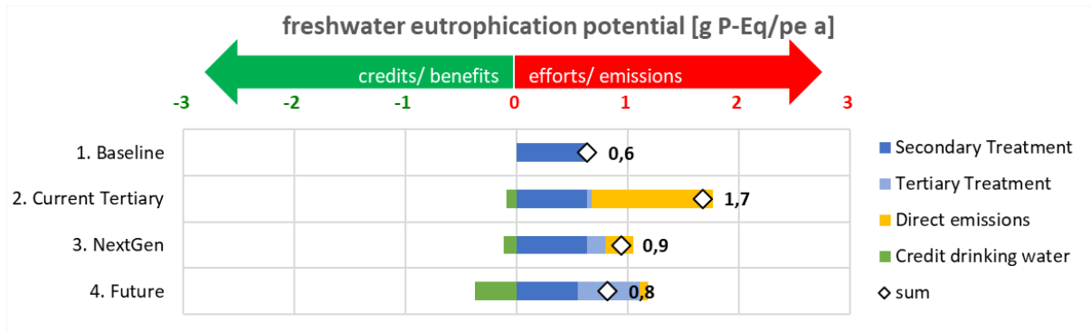
Figure 32: Freshwater eutrophication potential for the Tossa de Mar WWTP & WRP
