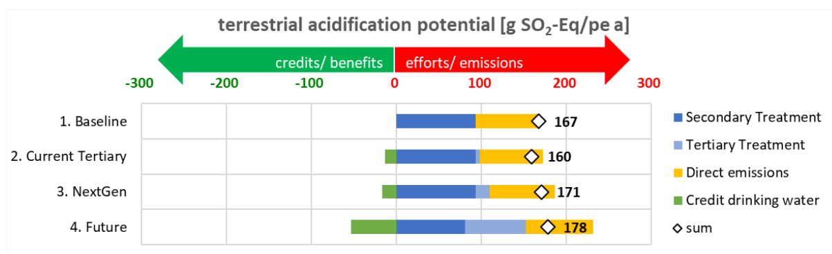
Figure 31: Terrestrial acidification potential for the Tossa de Mar WWTP & WRP
