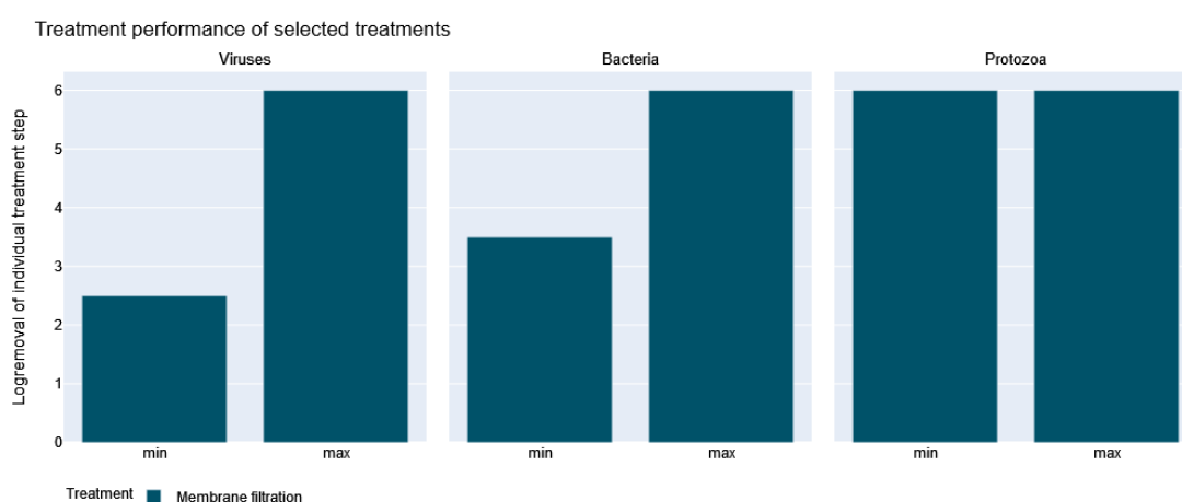
Figure 69: Overview of applied LRV in Filton
