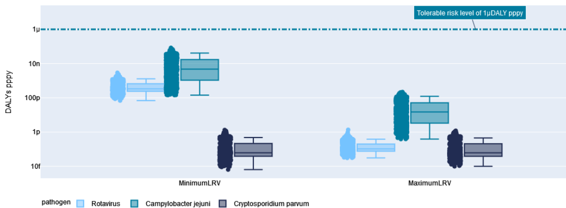
Risk in Disability adjusted life years (DALYs) per person per year (ppy)
