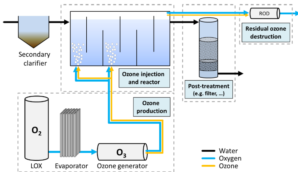
Figure 1: Scheme of a full-scale ozonation plant consisting of an ozone production unit, an ozone injection and reactor, an off-gas treatment, and post-treatment. Source: Stapf et al. (2020).
