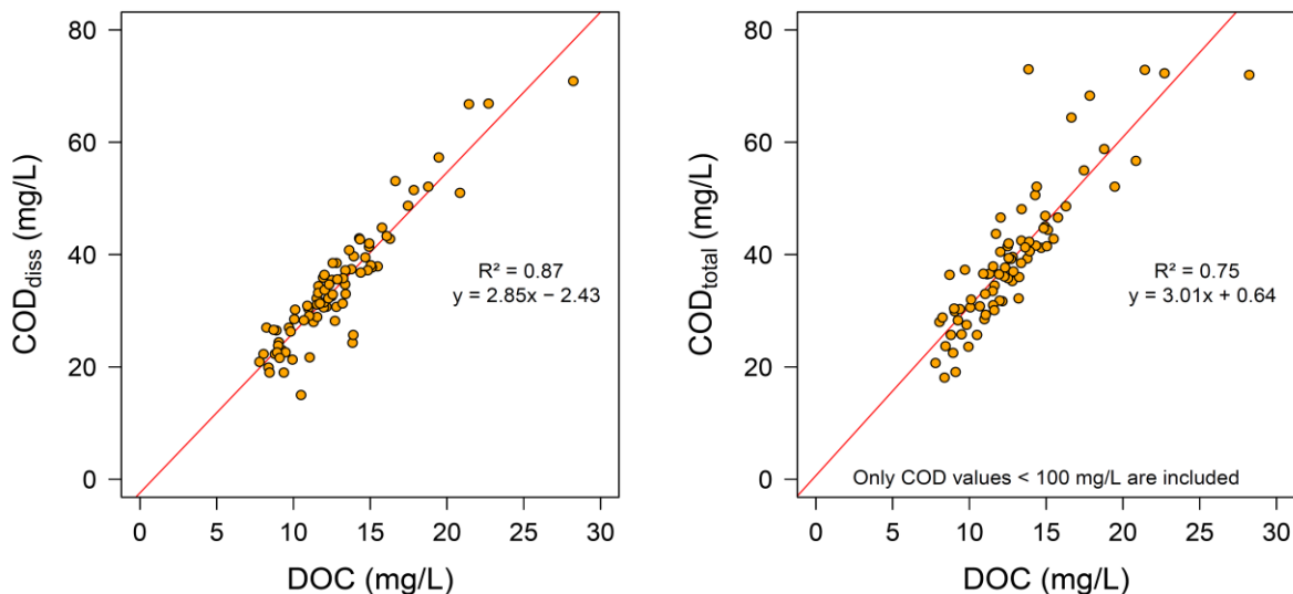
Figure 15: Correlation between DOC and total and dissolved COD.
