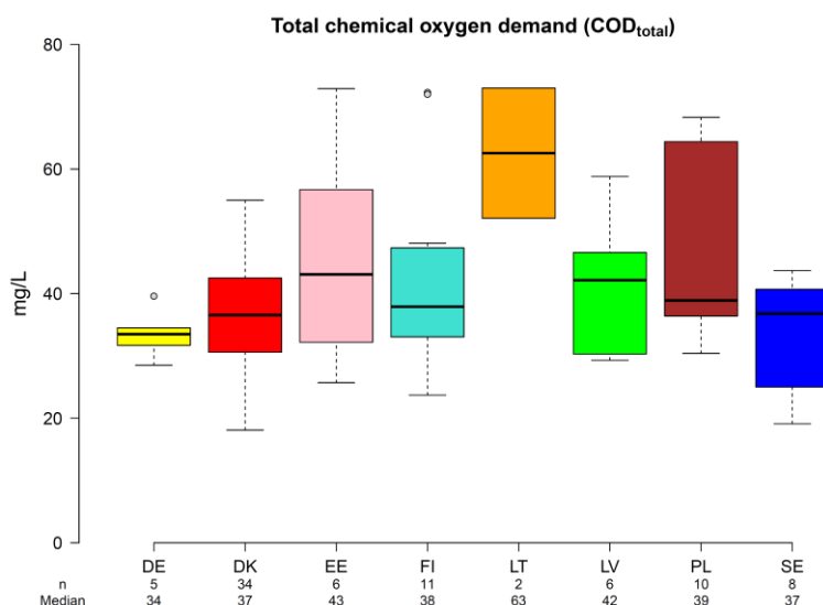
Figure 12: Total COD in analyzed samples.
