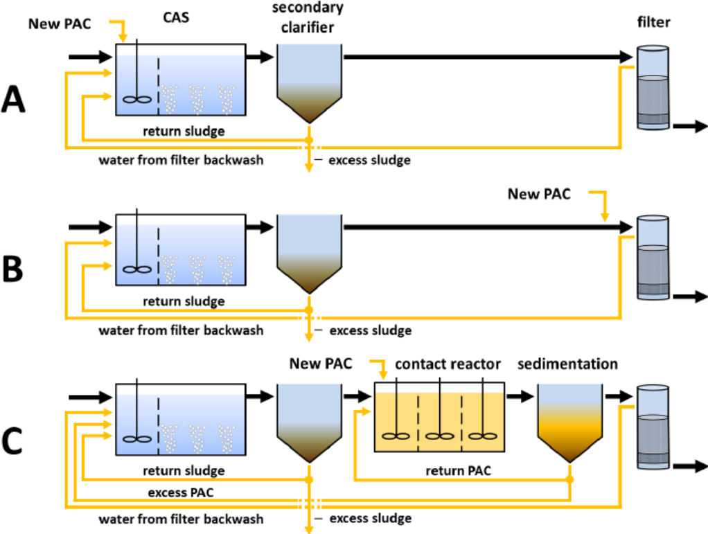
Figure 2: Schematic overview of different PAC processes which have been applied at full-scale plants: A) simultaneous PAC dosage, B) PAC dosage prior to a filter, and C) separate PAC contact reactor (“Ulmer process”). Source: Stapf et al. (2020).
