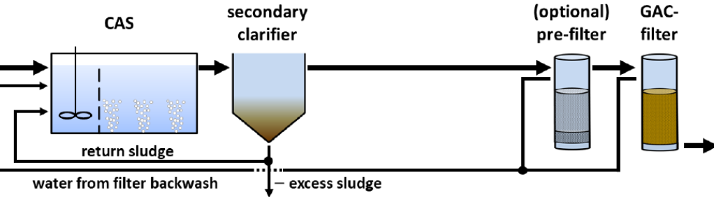
Figure 3: Scheme of a full-scale GAC process. Source: Stapf et al. (2020).
